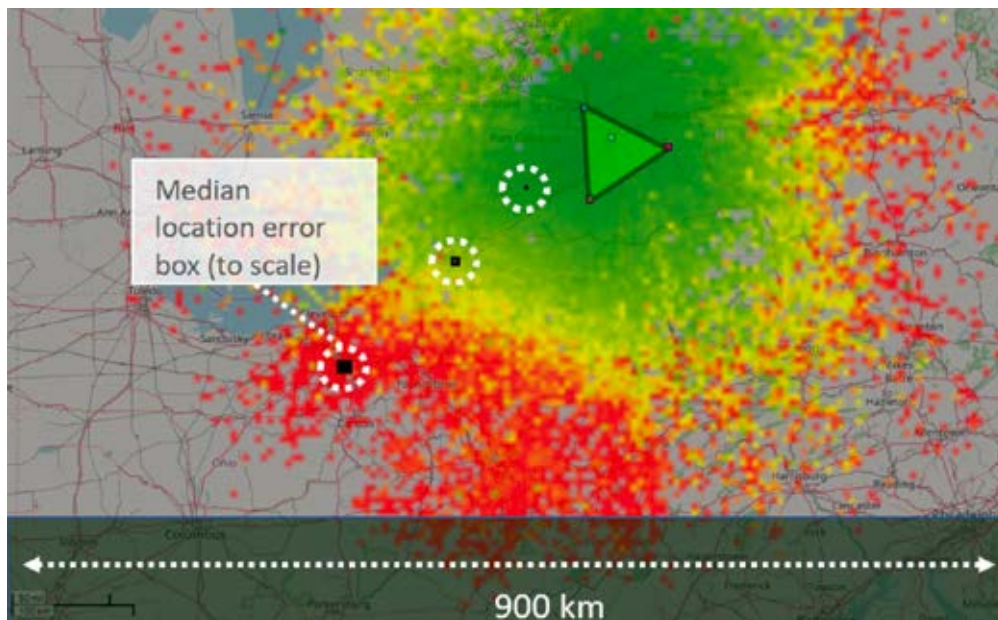
<< Figure 6 Comparison of 3D TDOA with ADS-B locations
