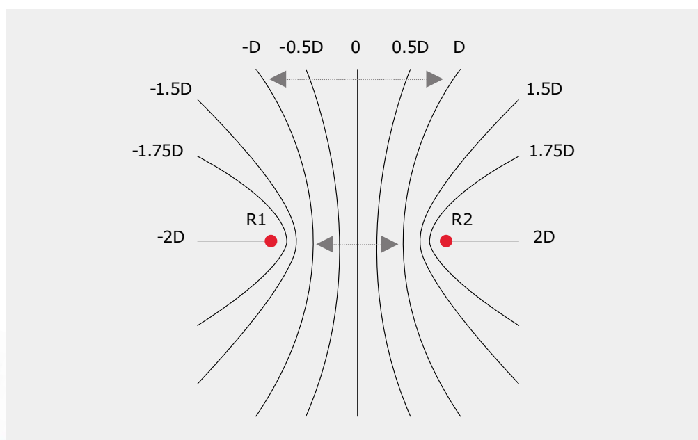
<< Figure 4 Effects of emitter position on x-coordinate uncertainty
