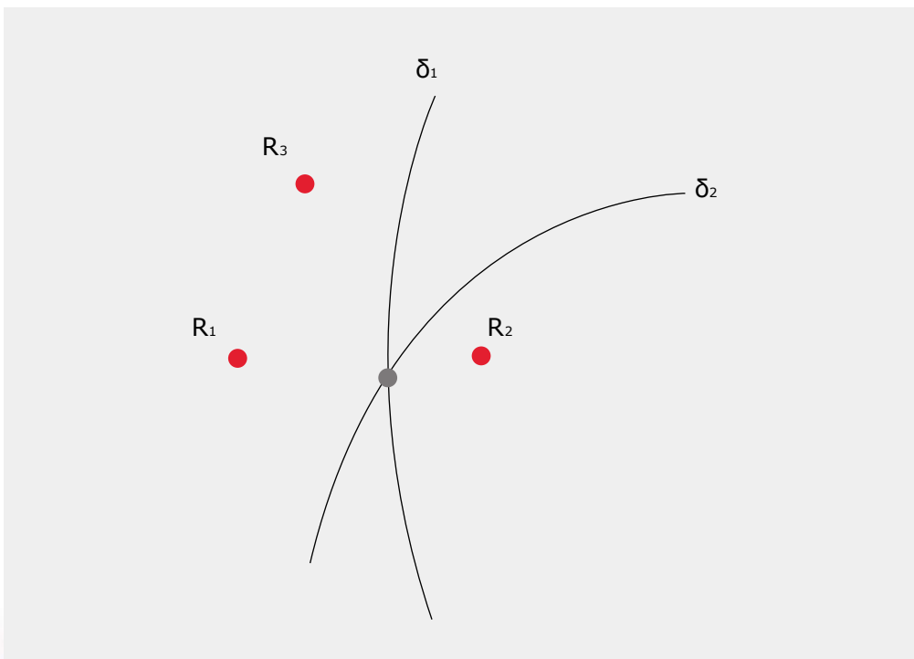
<< Figure 3 Two hyperbolas intersect at the source location
