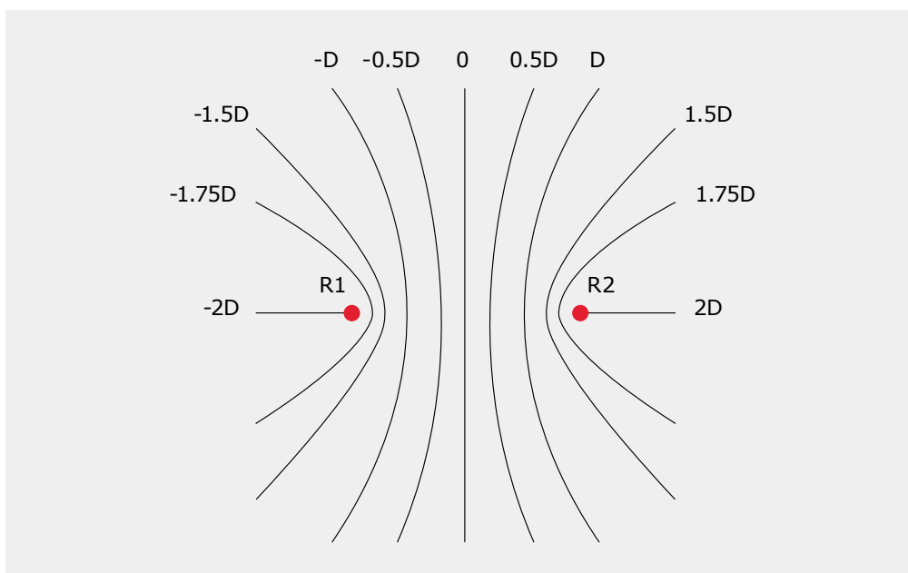
<< Figure 2 Curves indicating possible transmitter locations that correspond to various values of \delta_1
